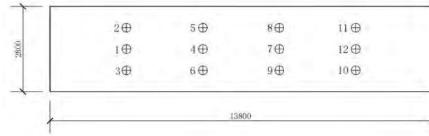
Figure 3 — Deflection measurement point layout plan
