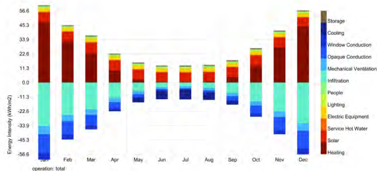
Figure 5 — Modified energy balance diagram
