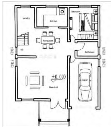
Fig.1 First-floor Plan
