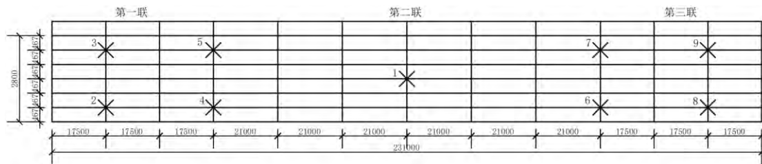
Figure 4 —Acceleration sensor measurement point layout diagram
