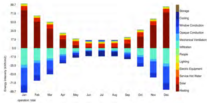
Figure 4 — Energy balance diagram before renovation
