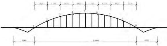
Figure 2— Strain measurement point diagram
