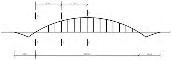
Figure 1— Schematic diagram of the load test control section
