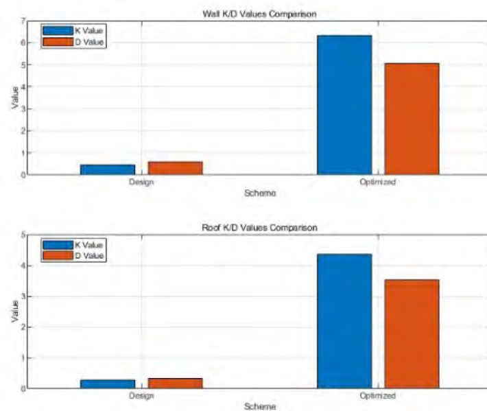
Figure 3. Wall K/D Values ~ Roof K/D Values Comparison
